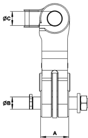
Single swing damper 80-184 M52 3T
