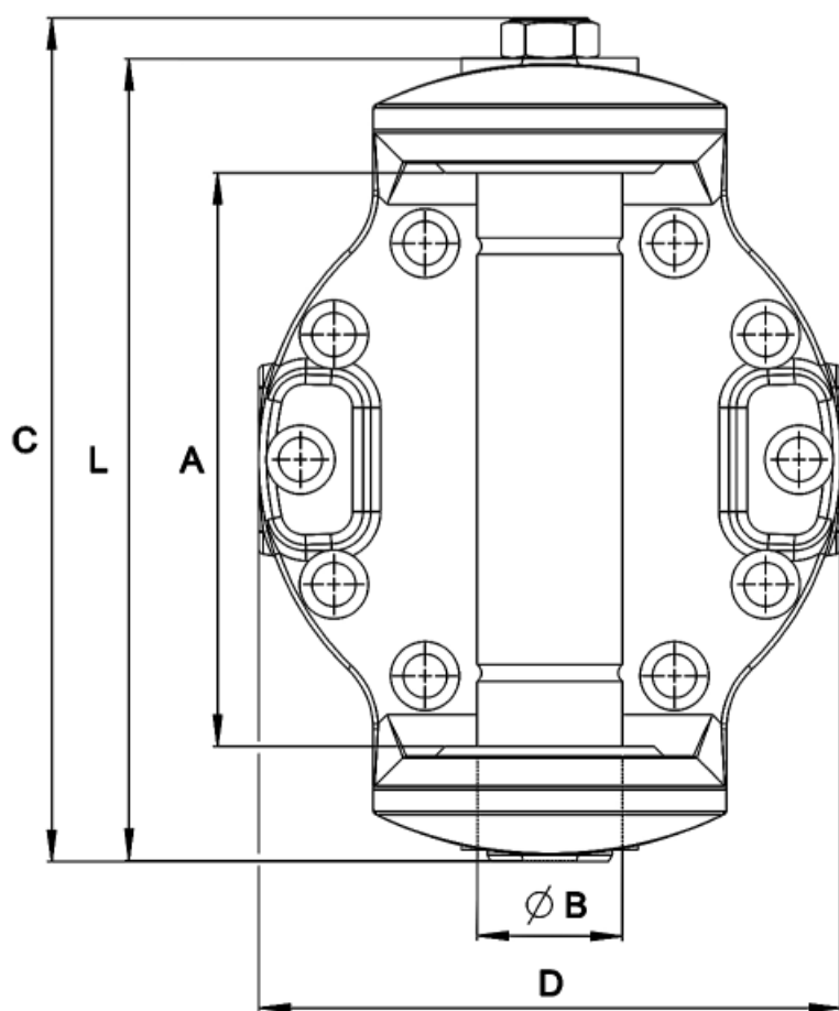
Mounting IR 22 /XR 400 I
